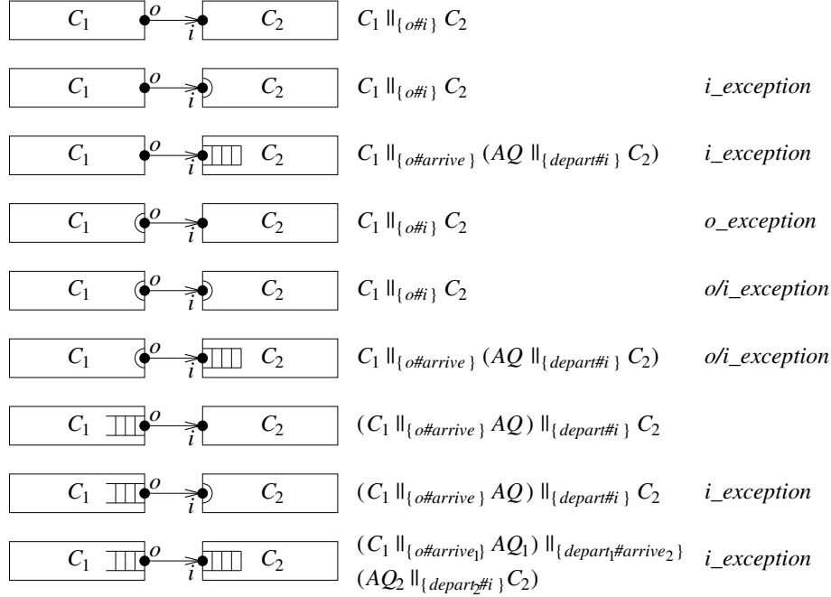
Figure 3.1. Synchronous, semi-synchronous and asynchronous communications
