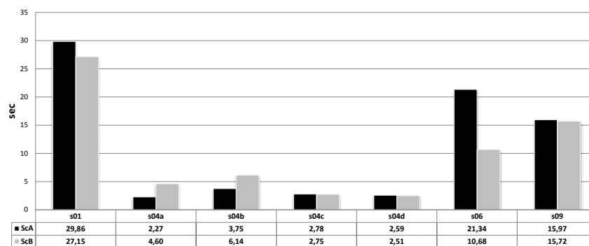
Fig. 22 New contributions to the average response times of standard RPD service - HP Set.
