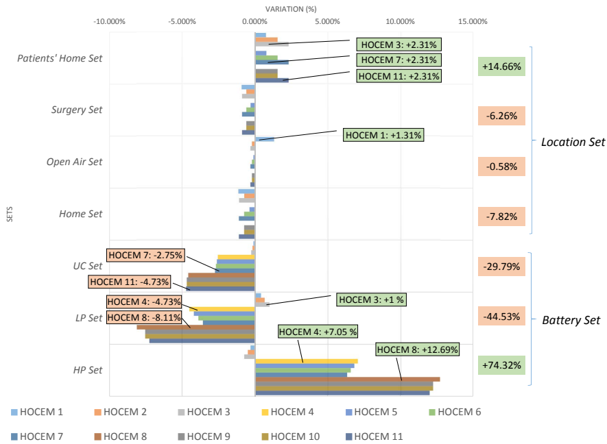
Fig. 8 Sensitivity analysis: sojourn probability variations in ScA.
