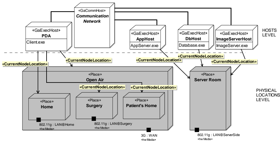
Fig. 13 The MeH Dynamic Deployment Diagram.
