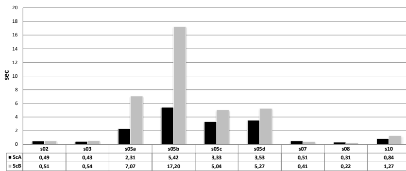
Fig. 21 Contributions to the average response times of Resource Constrained RPD service - UC and LP Sets.
