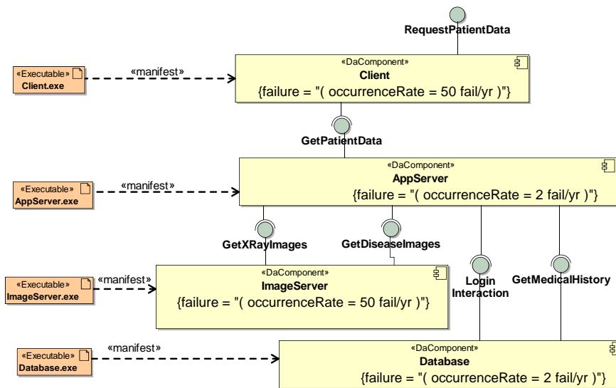
Fig. 11 The MeH software architecture.
