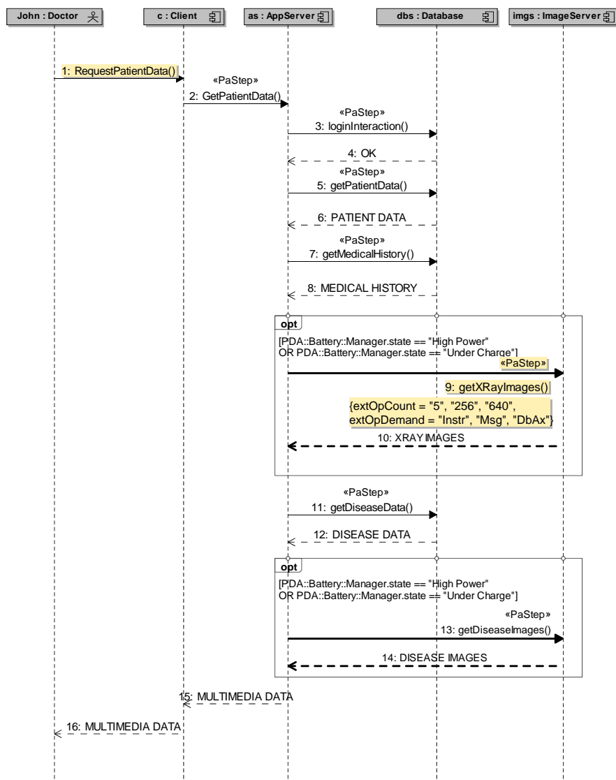
Fig. 12 The RPD Sequence Diagram.
