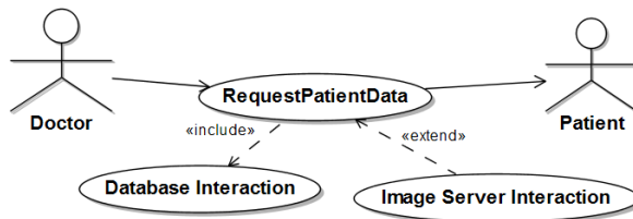
Fig. 10 The MeH Use Case Diagram.
