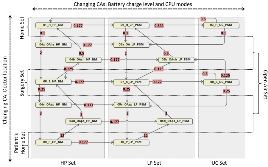
Fig. 5 The HOCEM for MeH parametrized with rates for ScA.
