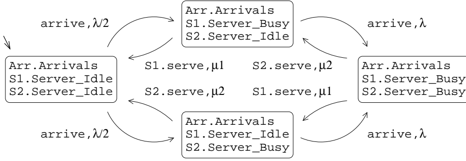
Fig. 1. ACTMC model of the queueing system example
